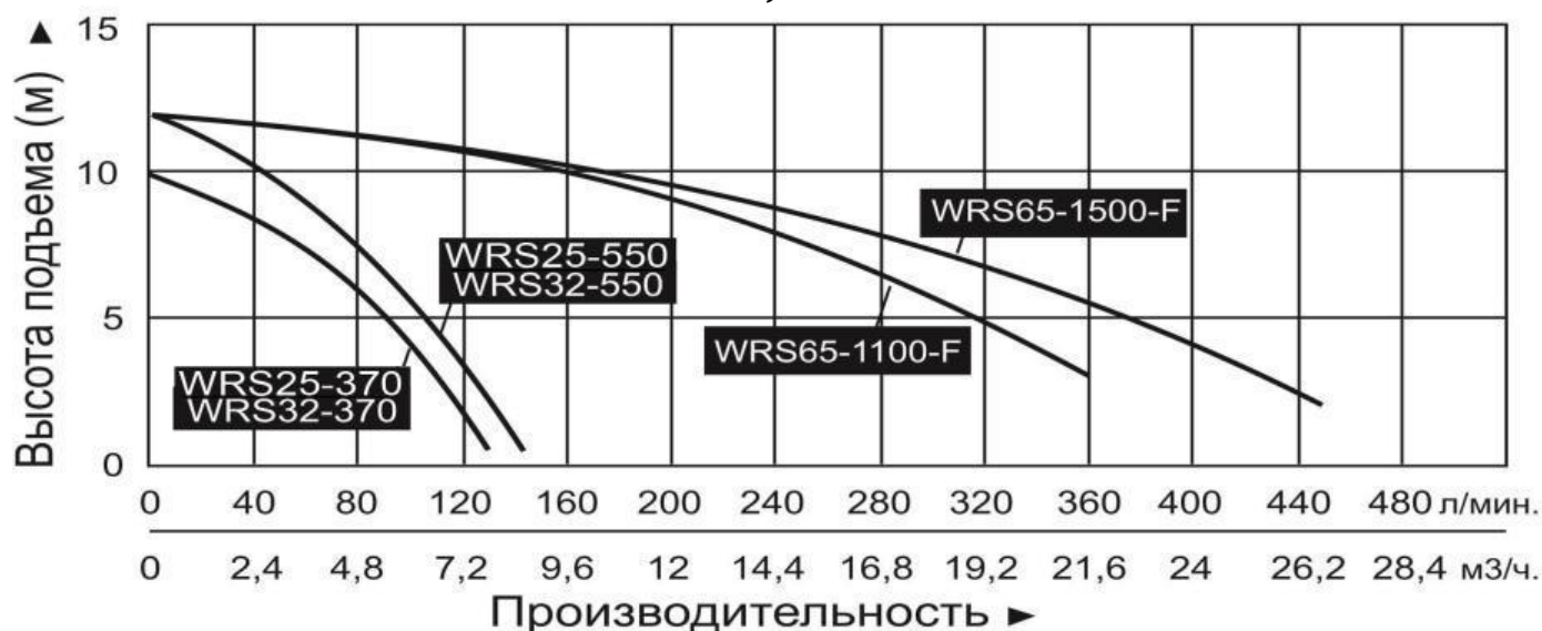
5.16. Модели WRS25-370, WRS32-370, WRS25-550, WRS32-550, WRS65-1100-F, WRS65-1500-F.
